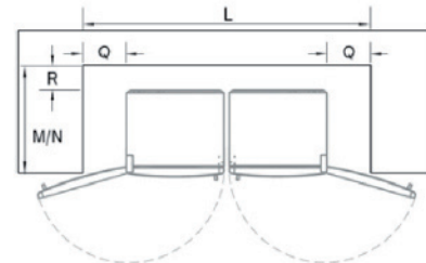
3. Flush with refrigerator door – full door rotation.
