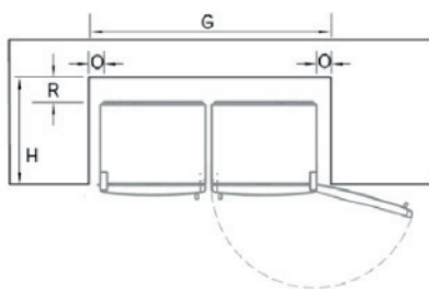
1. Flush with refrigerator chassis – full door rotation.
