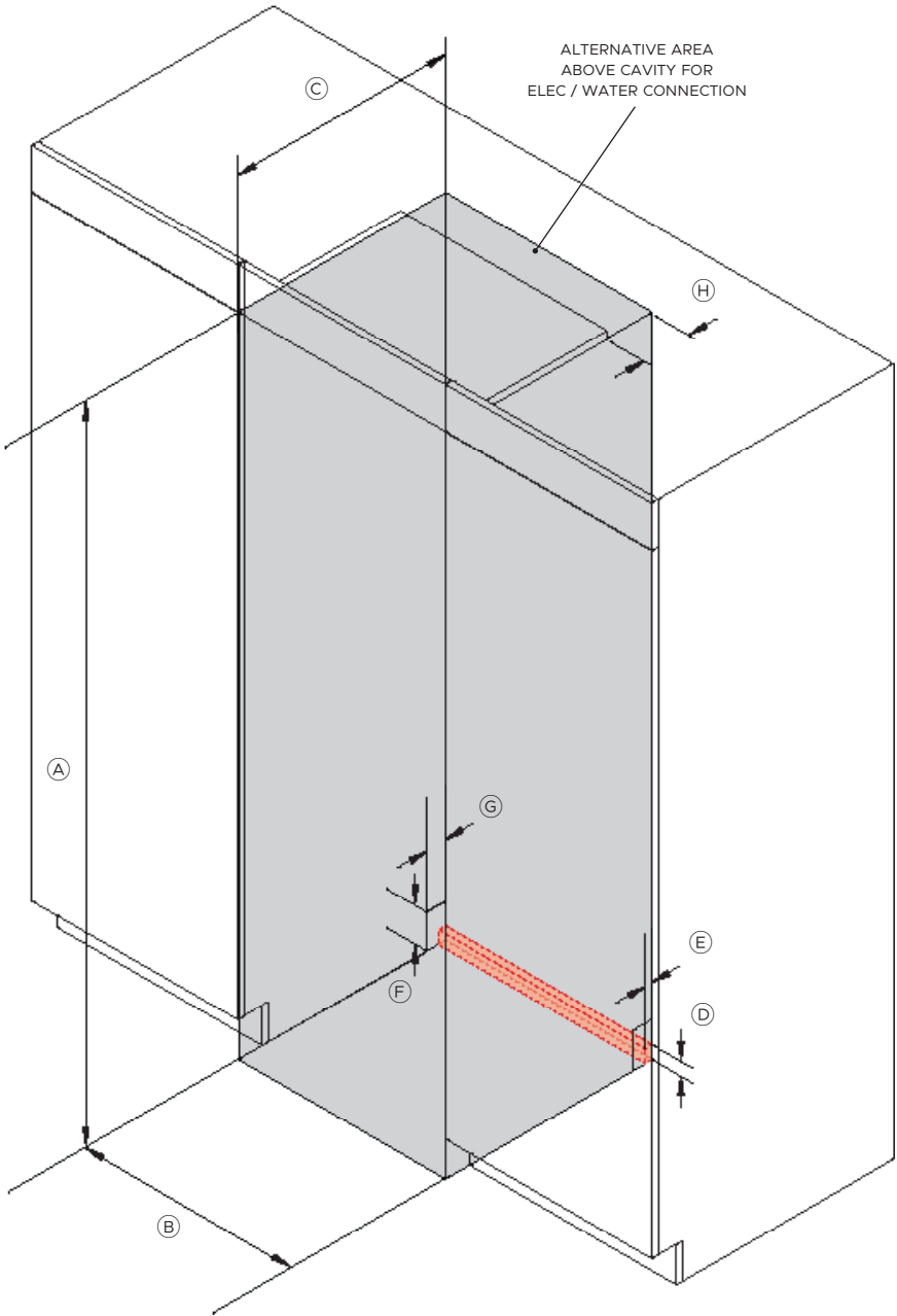
ISO VIEW
