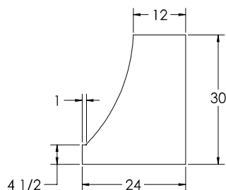
36" SIDE VIEW
