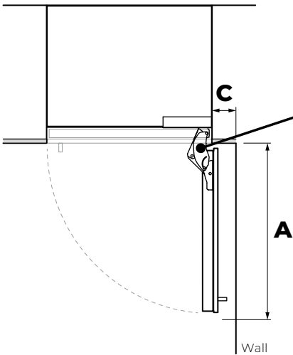
90° DOOR OPENING
