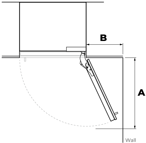
115° DOOR OPENING (FULL ROTATION)
