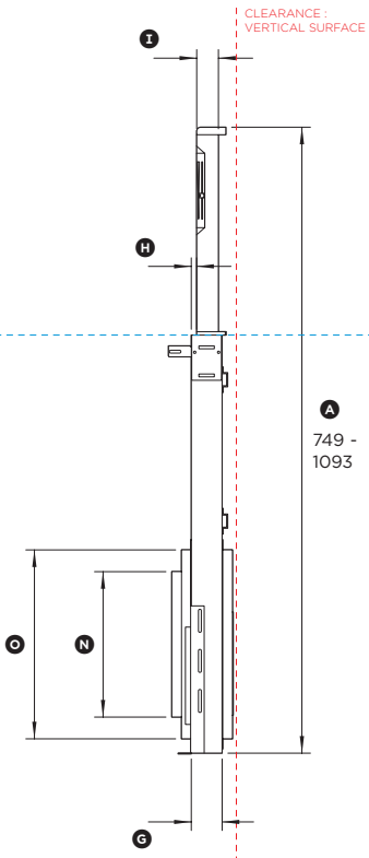
PROFILE VIEW
