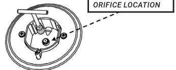
BURNER ORIFICE
