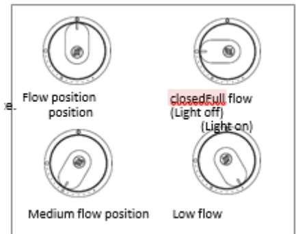
Figure 2: Control lever adjustment
