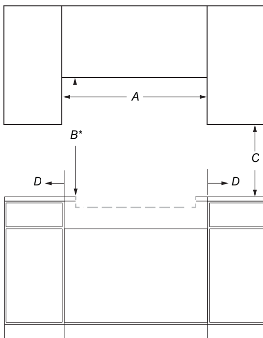
VISTA FRONTAL
