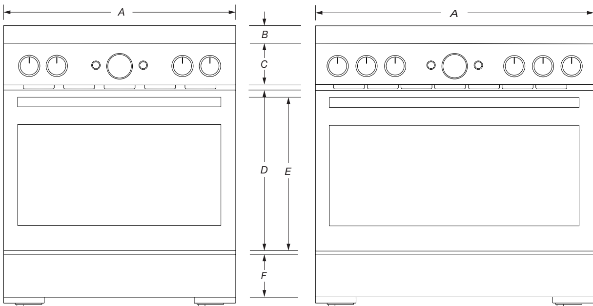
VISTA FRONTAL
