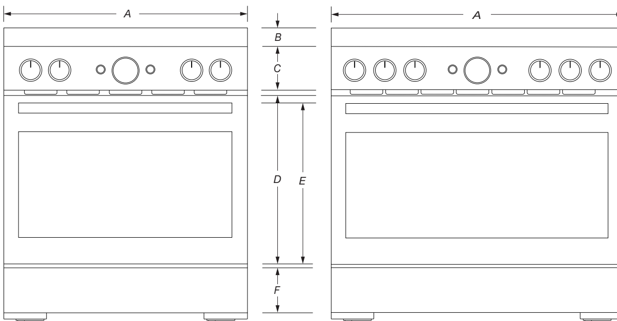
VISTA FRONTAL
