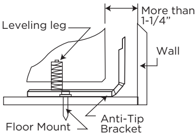
ANTI-TIP BRACKET (FLOOR MOUNTING ONLY)
