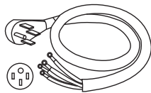
14-50P GETWIREDUSA FX359 (not applicable to products sold in Canada - these are provided with power cord)
